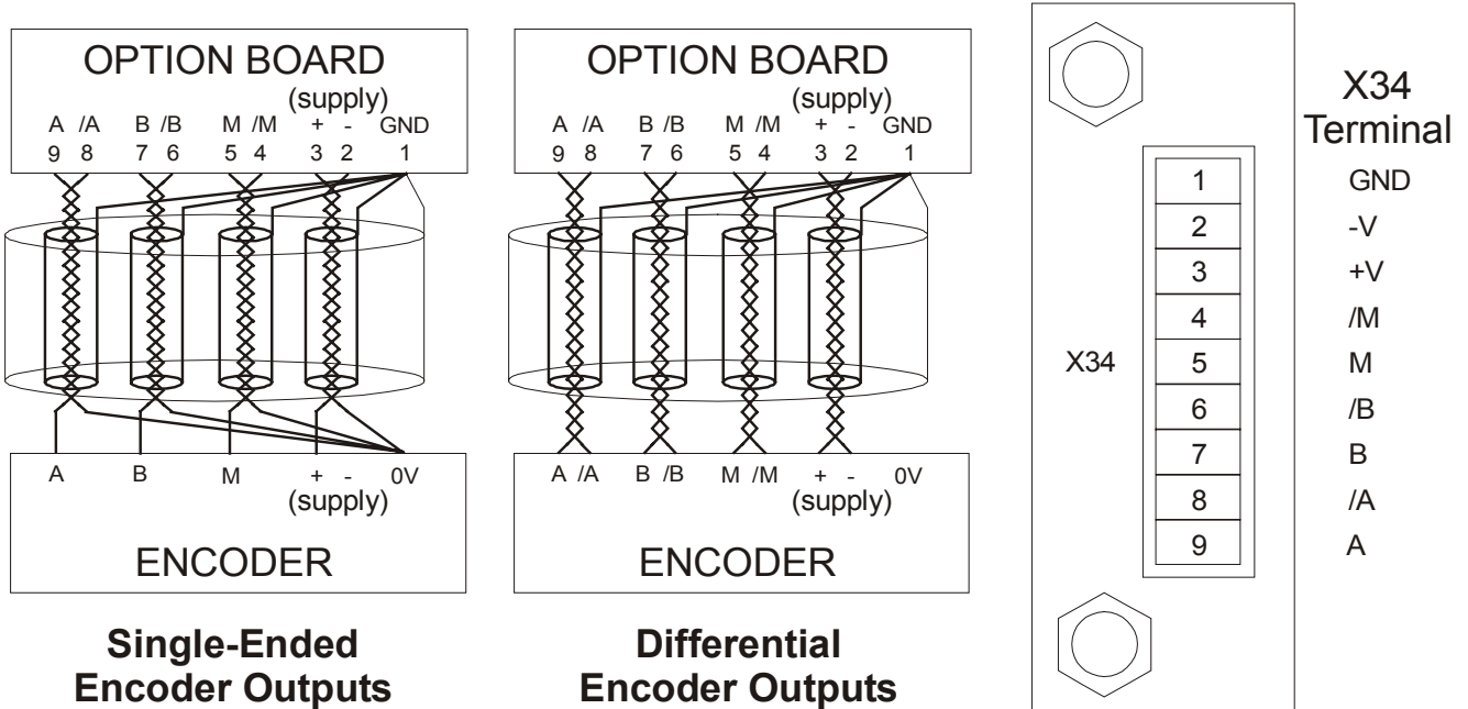
Figure 4 Wiring Diagram
