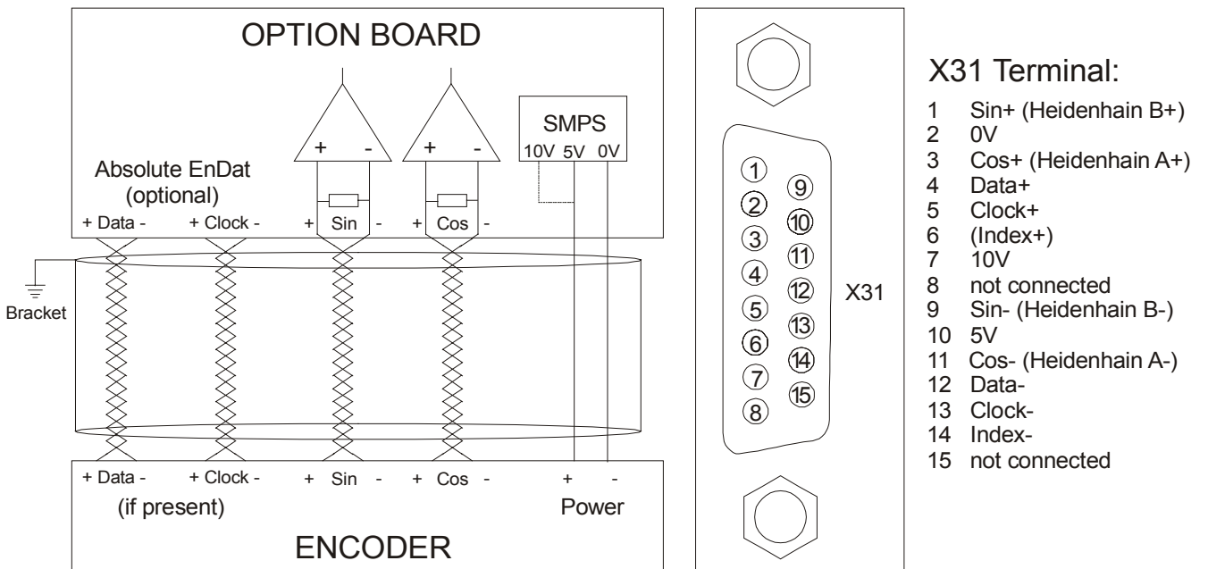
Figure 4 Wiring Diagram
